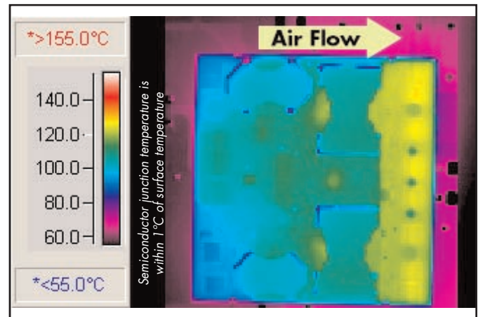
Figure 8: Thermal plot of converter at 37 amp load current with 55°C air flowing at the rate of 200 LFM. Air is flowing across the converter from input to output (nominal input voltage).
