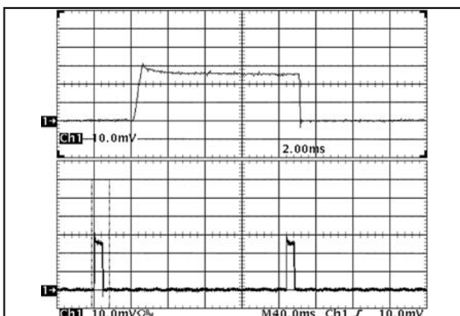
Figure 18: Load current (20A/div) as a function of time when the converter attempts to turn on into a 1\ m\Omega short circuit. Top trace (2ms/div) is an expansion of the on-time portion of the bottom trace.
