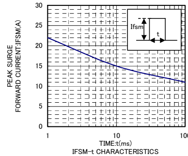
IFSM-t CHARACTERISTICS
