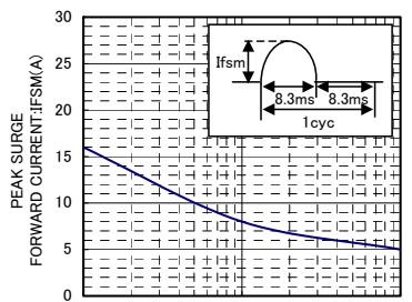
IFSM-CYCLE CHARACTERISTICS
