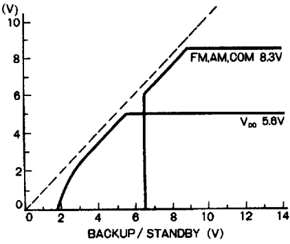
Figure 16 BA3906
