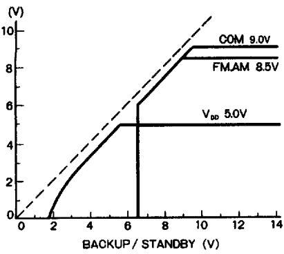
Figure 14 (BA3902)
