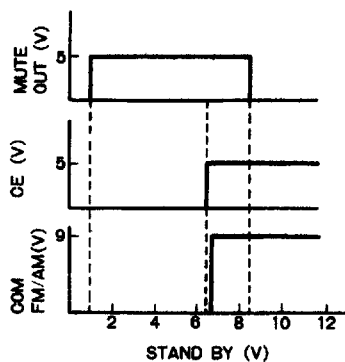
Figure 6 Standby (pin 8) 3.6 k \Omega
