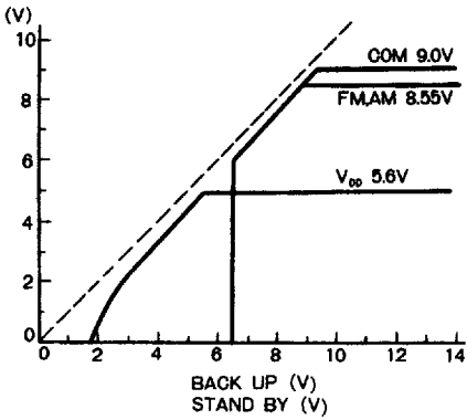
Figure 15 (BA3904A)
