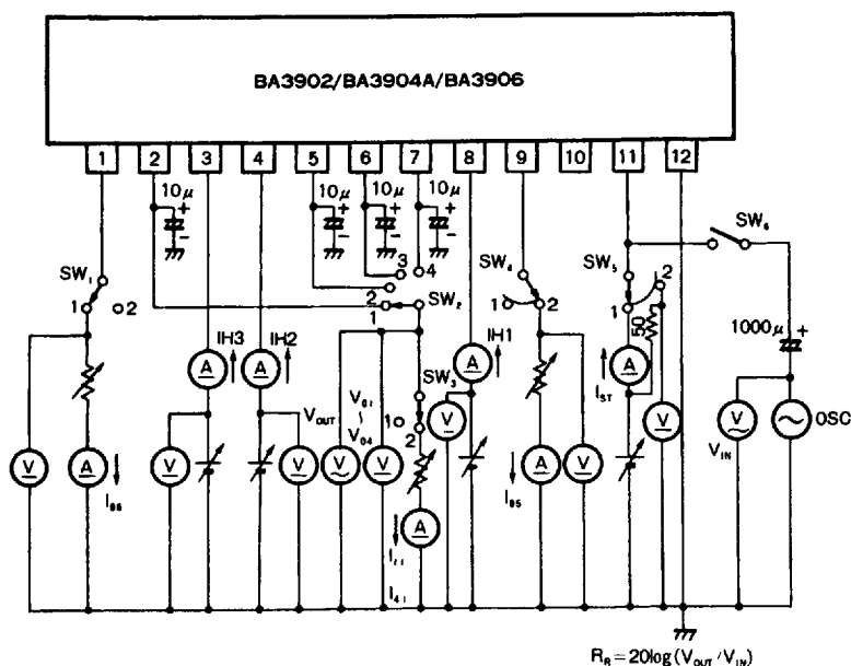
Figure 1 Test circuit
