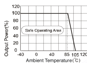
Temperature Derating Graph
