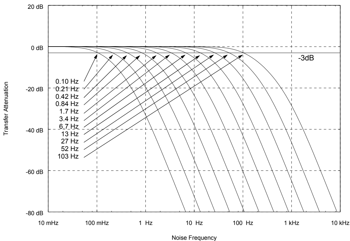
Figure 17: Noise Transfer Functions
