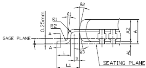
DETAIL "X" (20/1)
