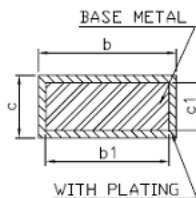
SECTION A-A WITH PLATING
