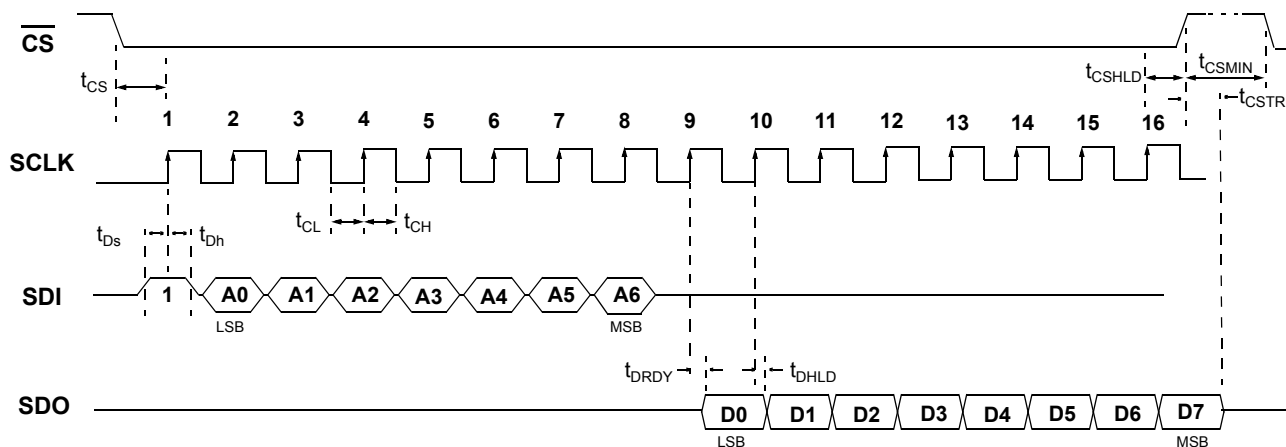
Figure 8: SPI Bus, Read access (Pin CLKE = Low)
