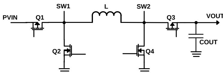
Figure 2 Buck-Boost Diagram
