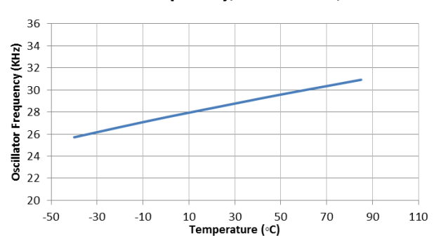
Oscillator Frequency, Vout=3.4V, USM
