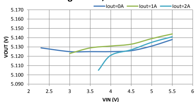
Line Regulation, V OUT =5.14V
