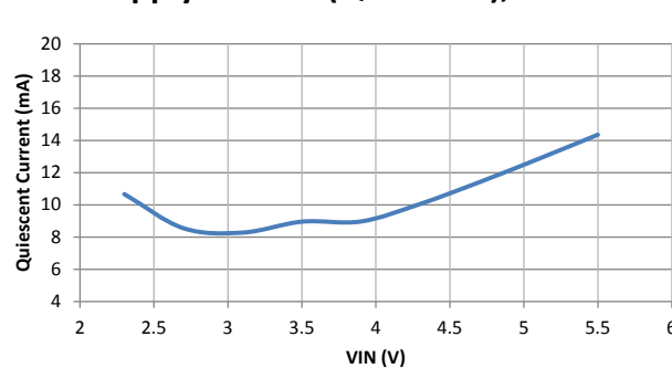
Supply Current (Quiescent), PWM
