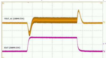
Load Transient (V IN =3V, PWM, I O =0A to 1A)
