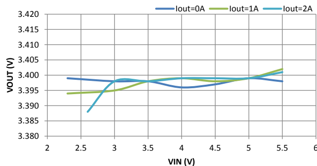
Line Regulation, V OUT =3.4V
