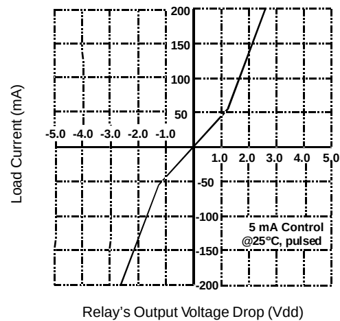
Figure 3. Linearity Characteristics
