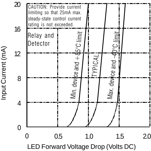
Figure 6. Input Characteristics (Current Controlled)
