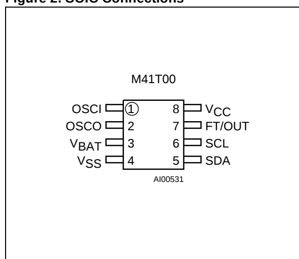
Figure 2. SOIC Connections
