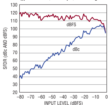
SFDR vs Input Level, f_{IN} = 70\text{MHz} , 20MSPS, 2V Range
