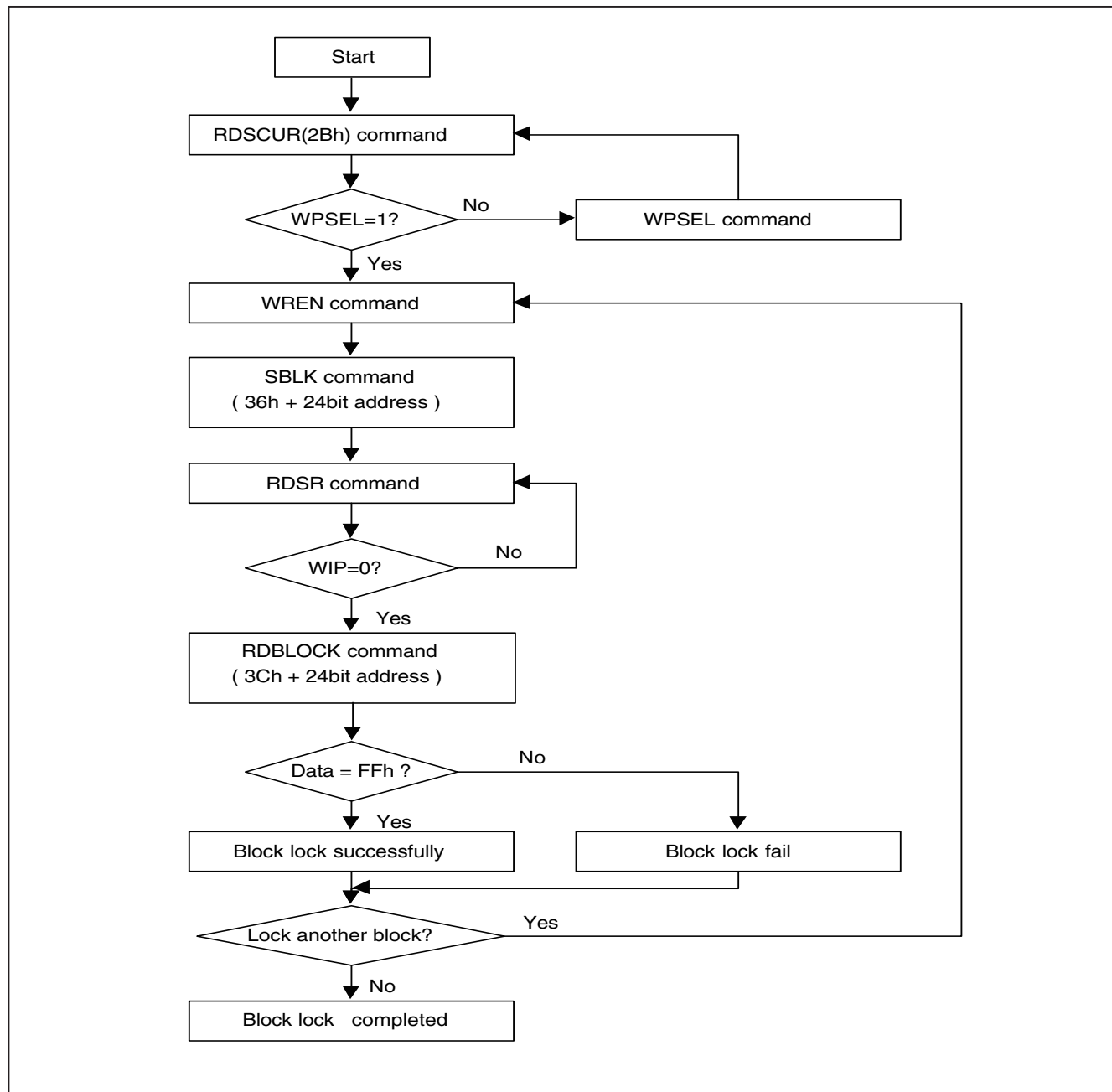
Figure 53. Block Lock Flow
