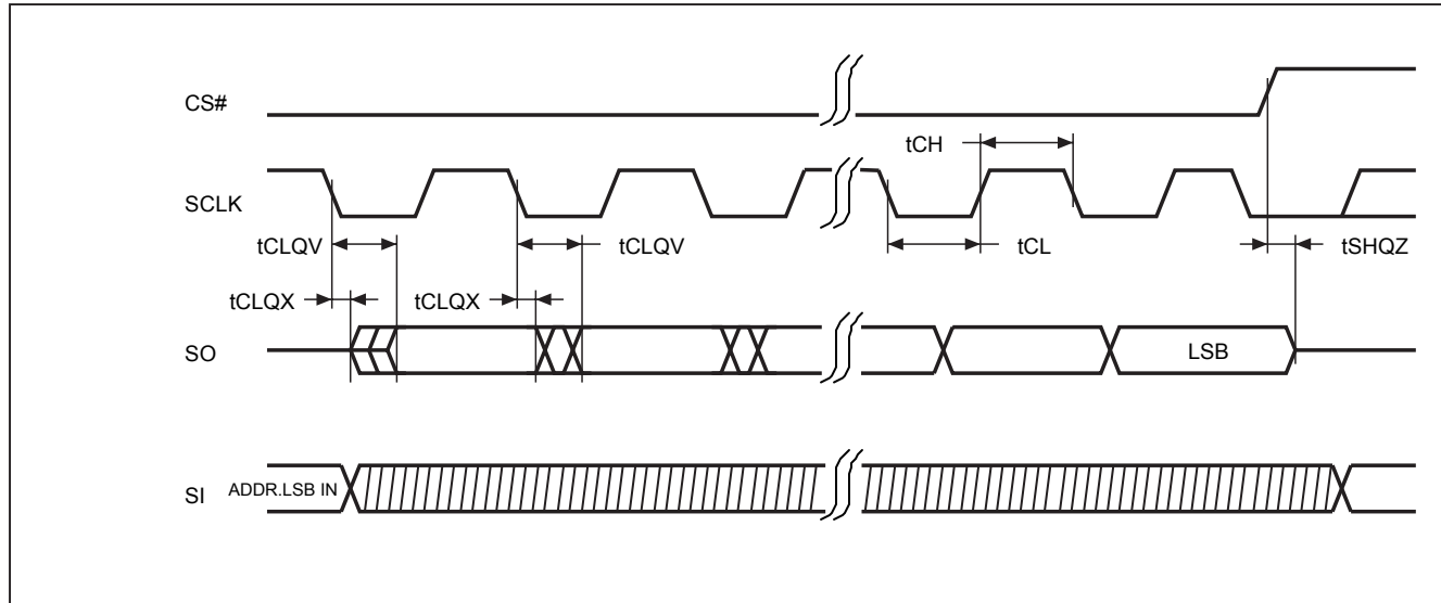
Figure 67. Output Timing
