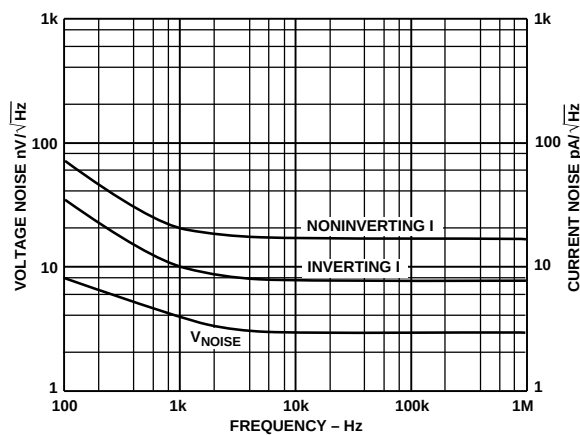
Figure 11. Input Current and Voltage Noise vs. Frequency
