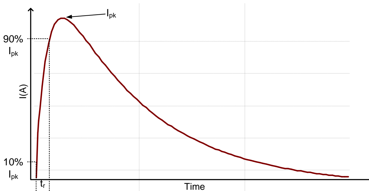
Figure 6. HBM Curve
