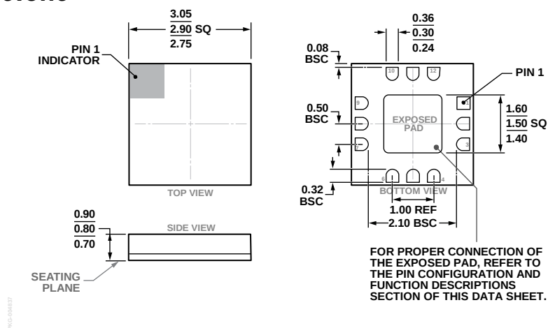
Figure 37. 12-Terminal Ceramic Leadless Chip Carrier (LCC) (E-12-4)
