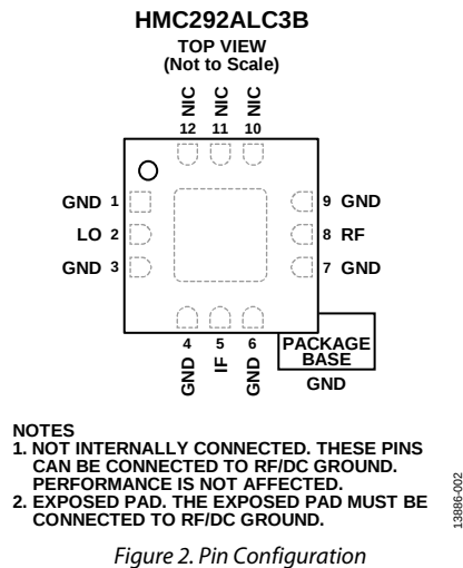
Figure 2. Pin Configuration
