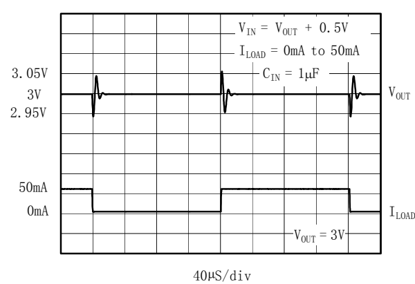
Load-Transient Response
