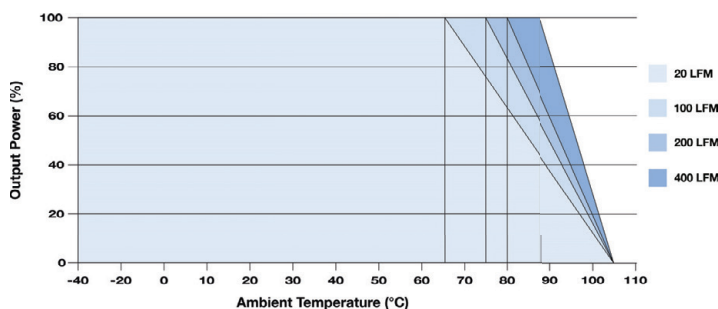
MB40xxS-05RU, MB4048S-12RU MB4048S-15RU Without Heatsink
