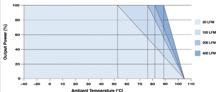
MB40xxS-24RU With Heatsink
