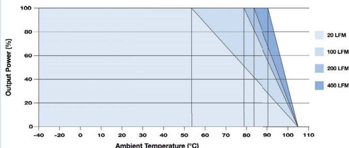
MB40xxD-12RU, MB40xxD-15RU With Heatsink
