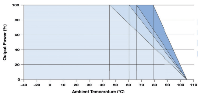
MB40xxD-12RU, MB40xxD-15RU Without Heatsink
