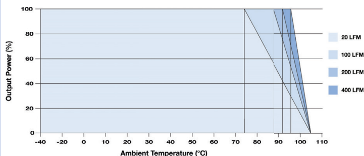
MB40xxS-05RU, MB4048S-12RU MB4048S-15RU With Heatsink
