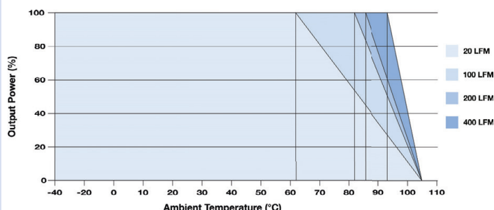
MB4024S-12RU, MB4024S-15RU With Heatsink
