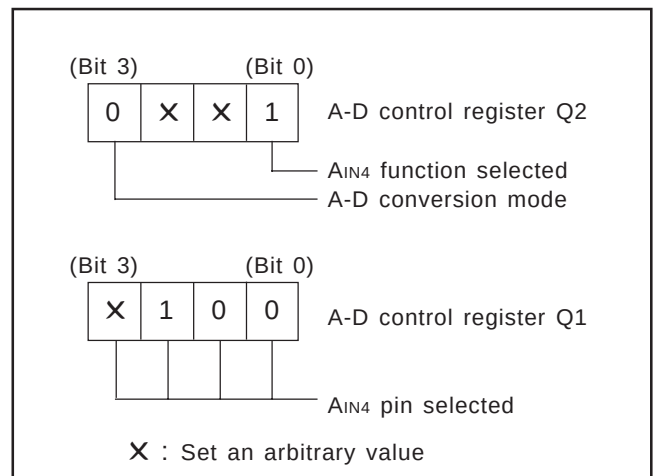
Fig. 28 Setting registers
