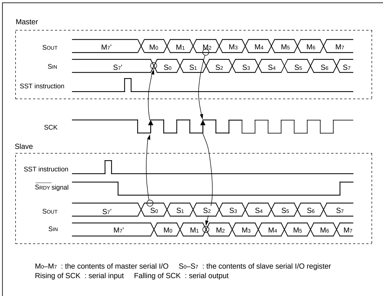
Fig. 25 Timing of serial I/O data transfer
