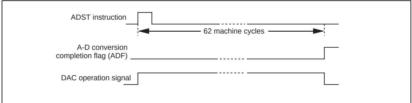
Fig. 27 A-D conversion timing chart
