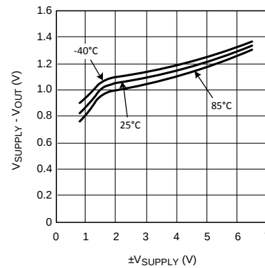
Figure 2. Positive Output Swing into 1\text{k}\Omega
