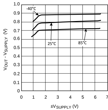
Figure 1. Output Swing R_L = 25\Omega, 1\text{k}\Omega @ -40^\circ\text{C}, 25^\circ\text{C}, 85^\circ\text{C}
