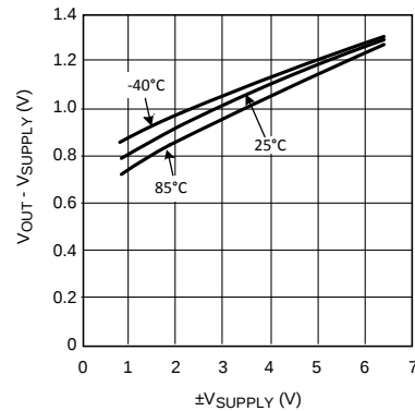
Figure 3. Negative Output Swing into 1\text{k}\Omega
