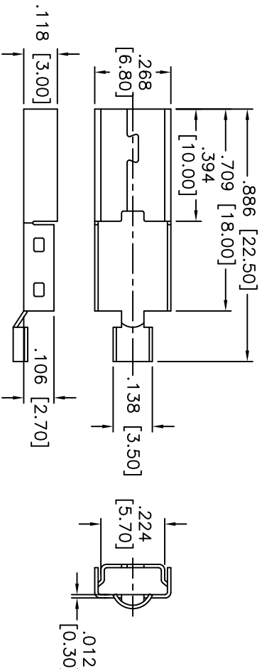
BACK SHELL
