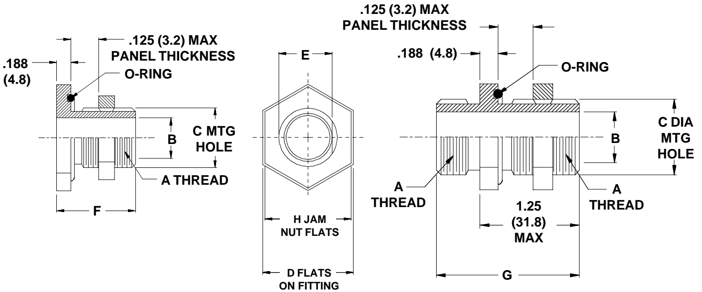
Bulkhead Adapters 710-100/101/372
