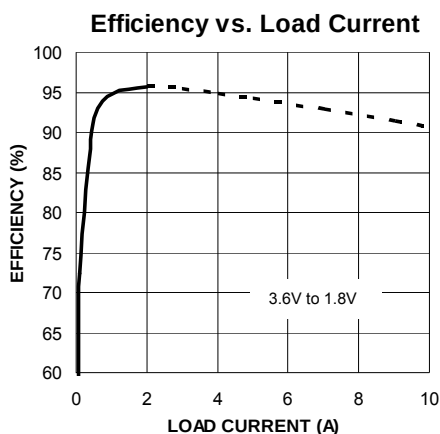
Figure 1. Efficiency Curve
