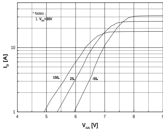
Fig.5 Transfer Characteristics
