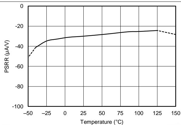
Figure 12. Power-Supply Rejection Ratio vs Temperature
