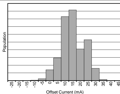
Figure 2. INA250A2 Input Offset Distribution
