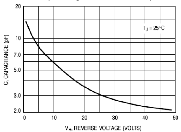
Figure 10. Typical Capacitance
