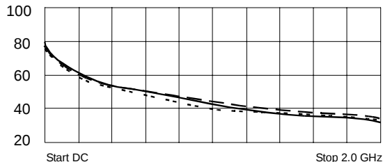
Isolation (dB)
