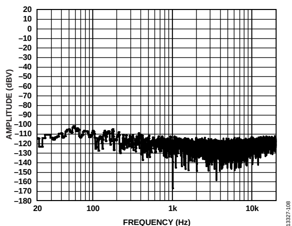
Figure 14. FFT, No Signal, Analog Gain = 15, R_L = 4\ \Omega
