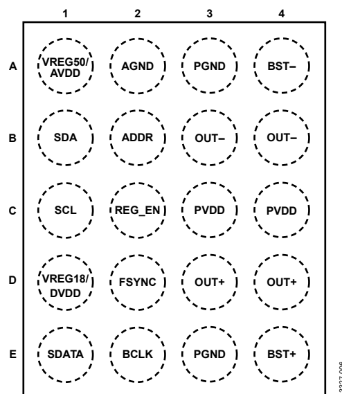
Figure 6. Pin Configuration (Top Side View)
