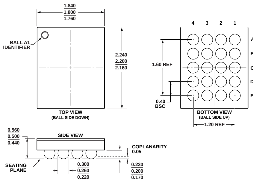
Figure 76. 20-Ball Wafer Level Chip Scale Package [WLCSP] (CB-20-10)
