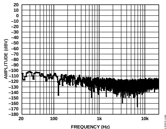
Figure 11. FFT, No Signal, Analog Gain = 8.4, R_L = 4\ \Omega
