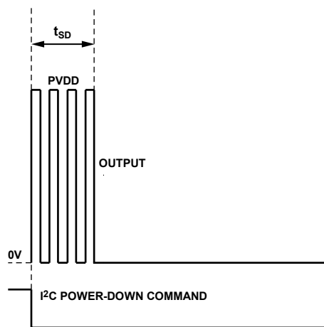
Figure 5. Turn Off Hard Volume
