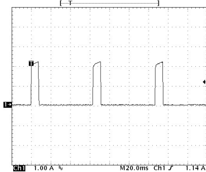
Short Circuit-Current
