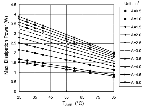
G1084T53(TO-263) Max. Power Dissipation vs. T_{AMB} (still air) ( Different PCB Top Copper Area )
