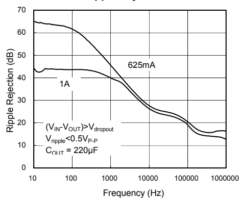
Ripple Rejection
