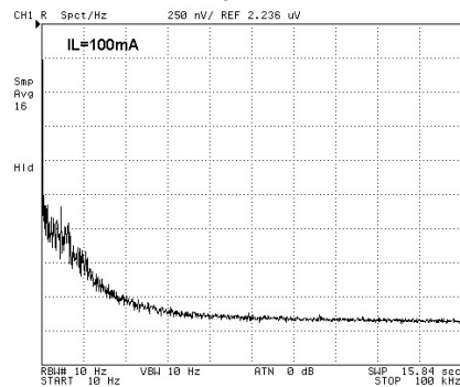
Output Noise
