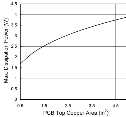
G1084T53(TO-263) Max. Power Dissipation vs. PCB Top Copper Area T_{AMB} = 25^{\circ}\text{C} ; Still Air
