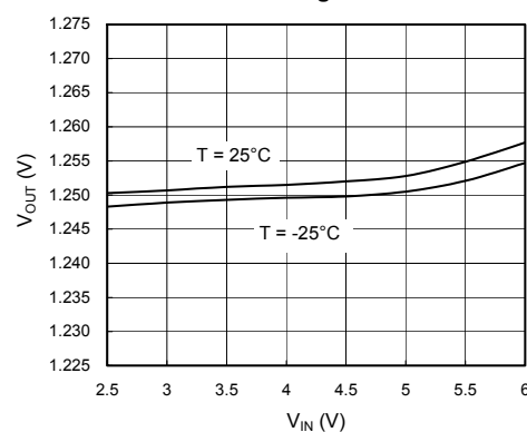
Line Regulation
