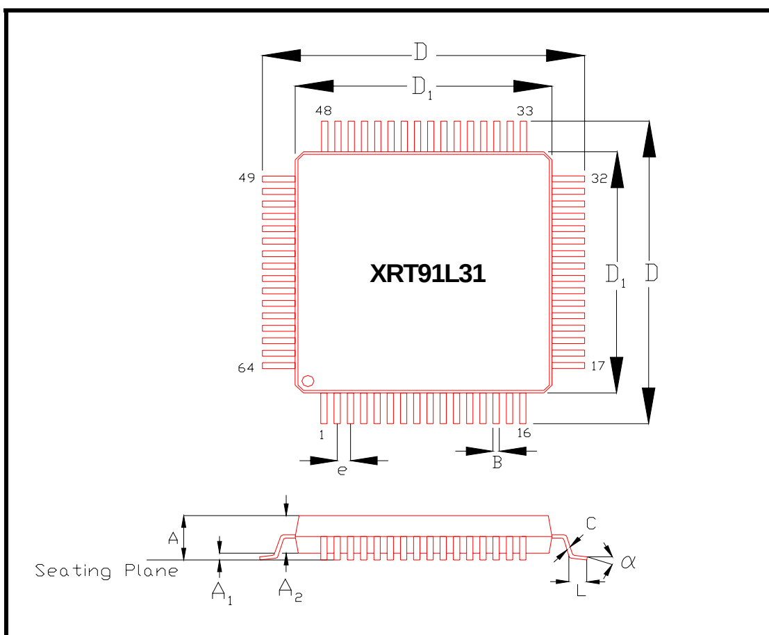
FIGURE 29. PACKAGE DIMENSIONS
