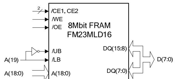
Figure 4. FM23MLD16 Wired as 1Mx8
