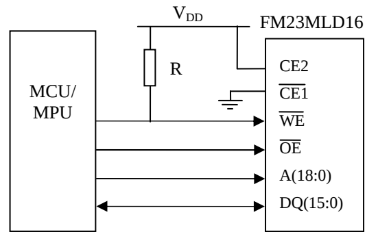
Figure 3. Use of Pullup Resistor on \overline{WE}
