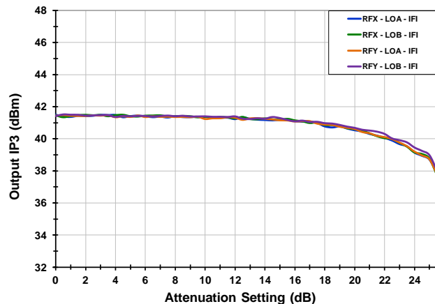
IP3 0 [1.0 GHz RF, HiSide Inj.]
