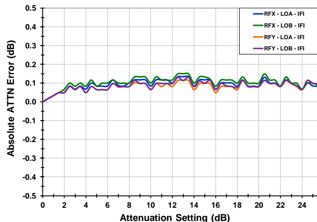
ATTN Accuracy [1.0 GHz RF, HiSide Inj.]
