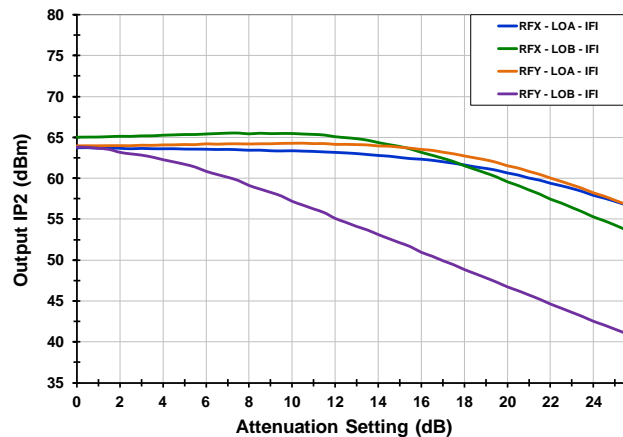
IP2 0 [1.0 GHz RF, HiSide Inj.]
