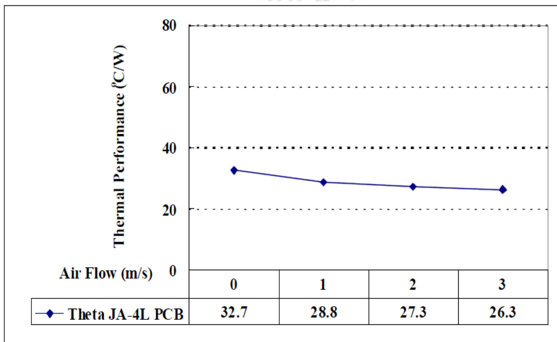
Thermal Performance of SLQFP under Forced Convection
