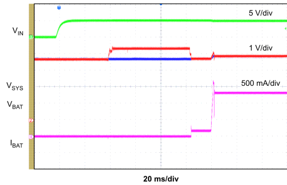
IN Plug-in with Battery Connected
