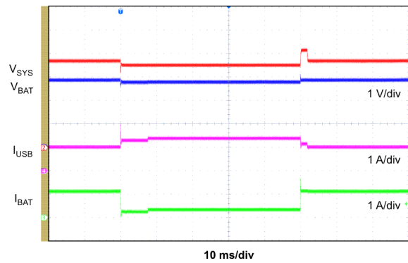
Load Transient into DPPM
