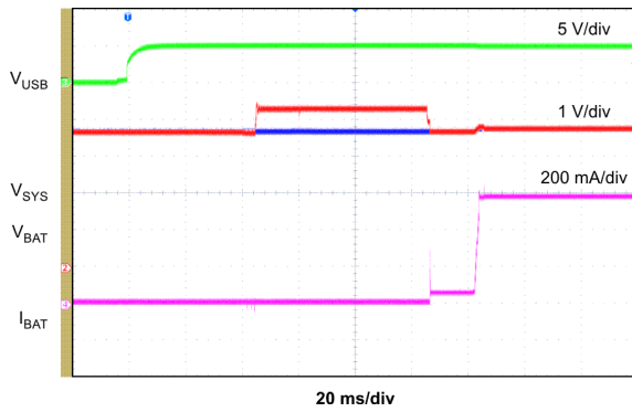
USB Plug-In with Battery Connected
