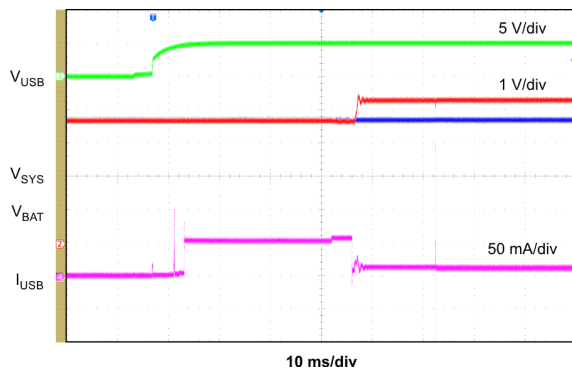
Adapter Detection USB
