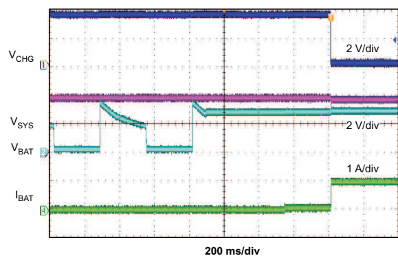
Battery Insert During Battery Detection
