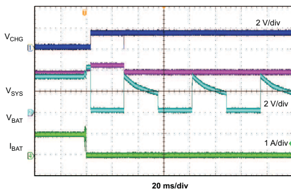
Battery Pull During Charging
