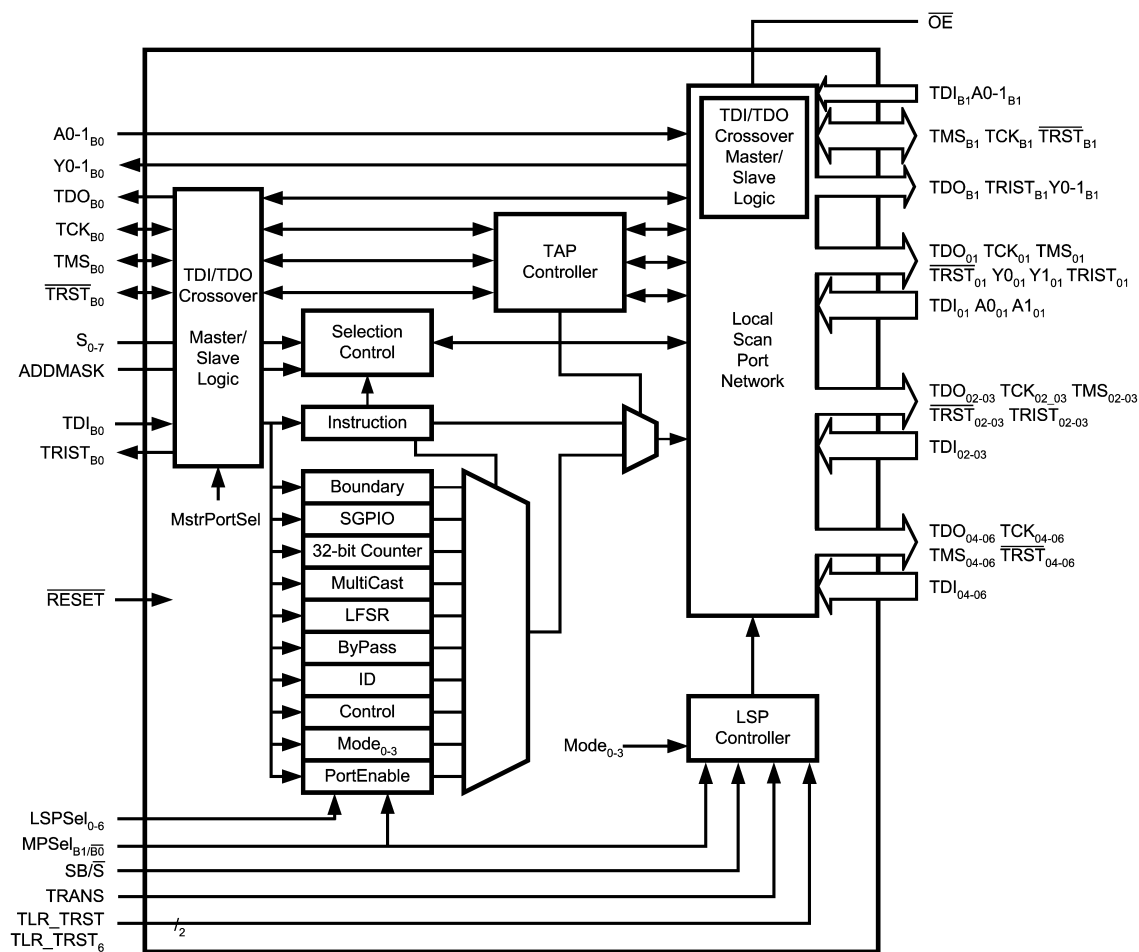
FIGURE 3. SCANSTA112 Block Diagram
