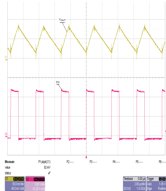
Figure 21. TPS54233 Output Ripple
