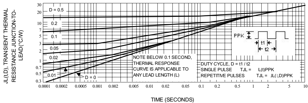
Fig. 3-TYPICAL THERMAL RESPONSE
