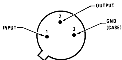
See NS Package Number H03A Bottom View
