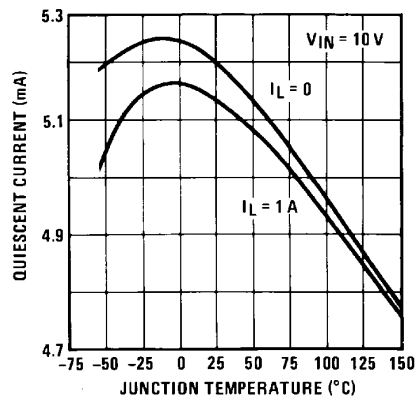
Quiescent Current
