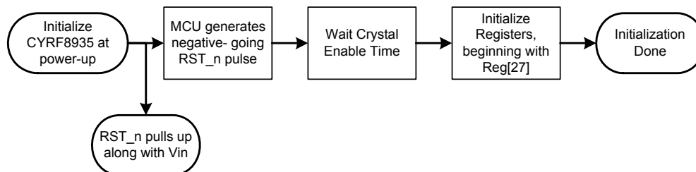
Figure 3. Initialization Flowchart
