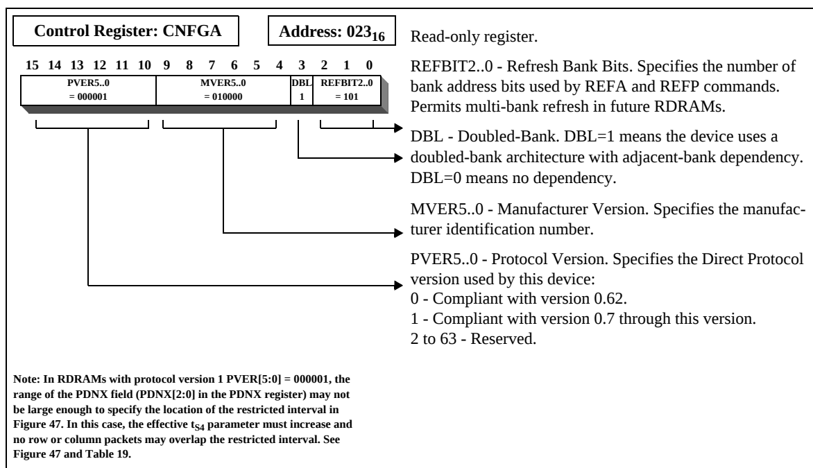
Figure 28: CNFGA Register
