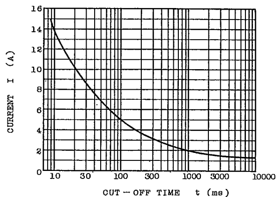
FUSE F_1 ; I-t CHARACTERISTIC
