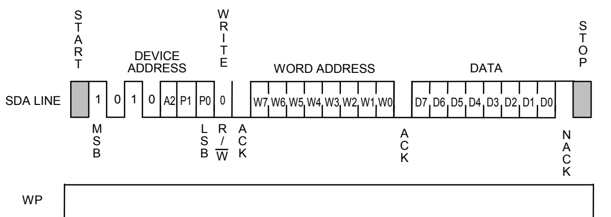
Figure 15 Write Protect
