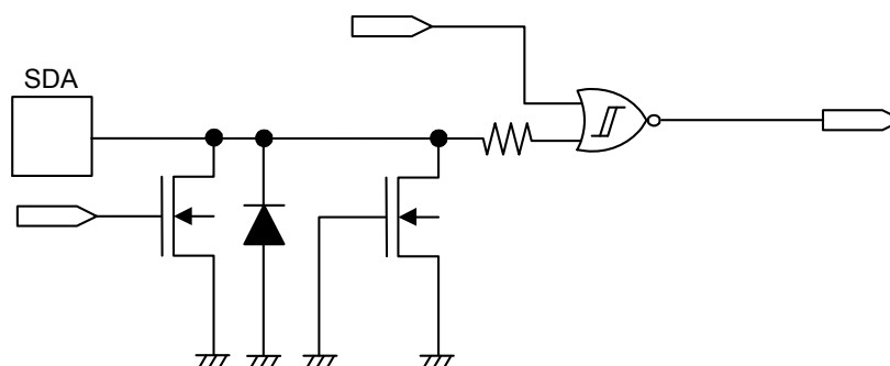
Figure 22 SDA Pin
