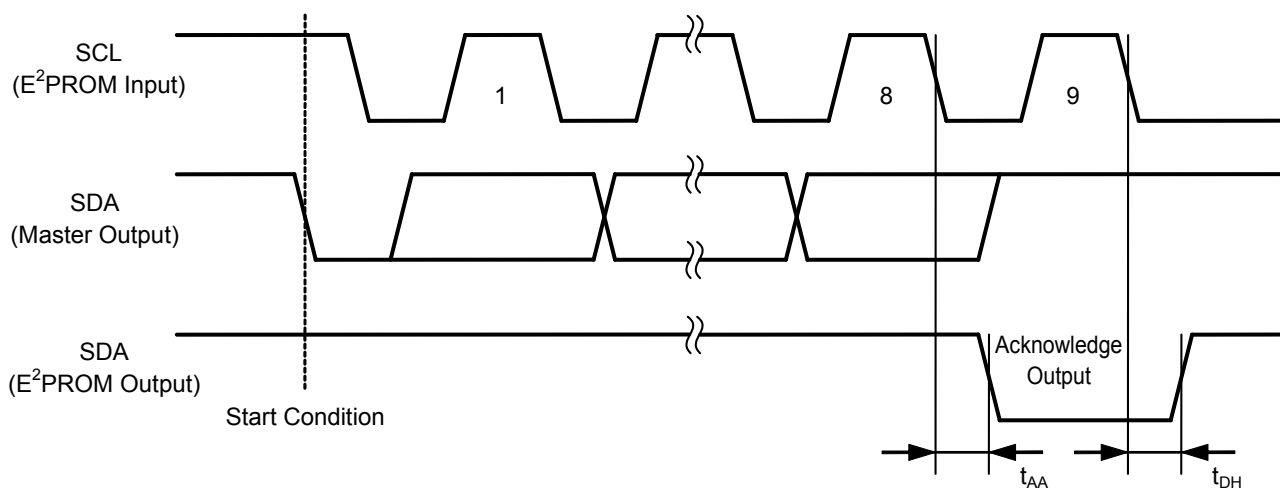
Figure 11 Acknowledge Output Timing
