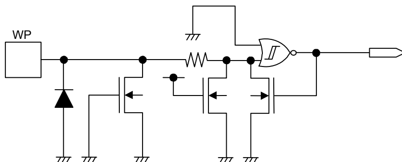
Figure 23 WP Pin
