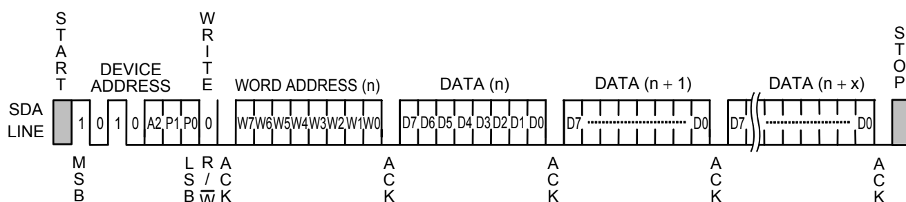
Figure 14 Page Write
