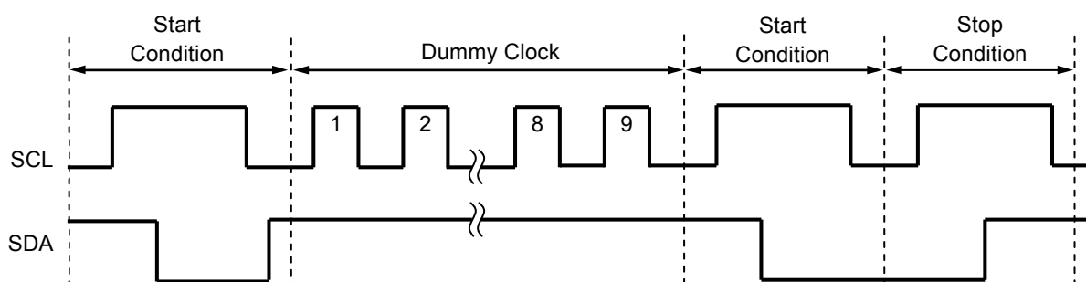
Figure 25 Resetting S-24C08C
