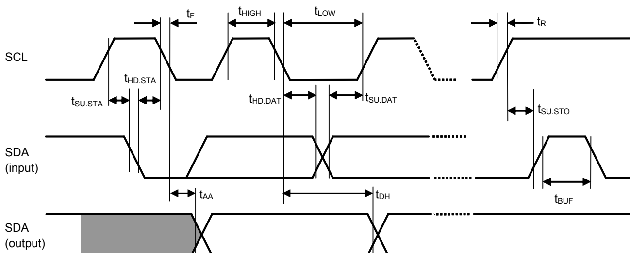
Figure 6 Bus Timing
