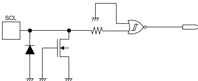
Figure 21 SCL Pin
