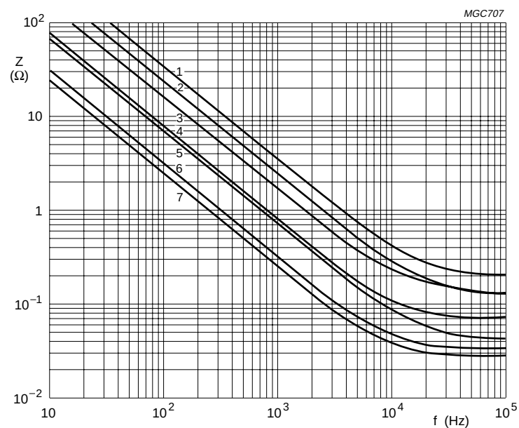
Fig.13 Typical impedance as a function of frequency.
