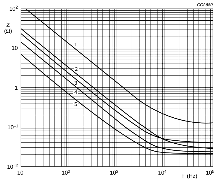
Fig.12 Typical impedance as a function of frequency.
