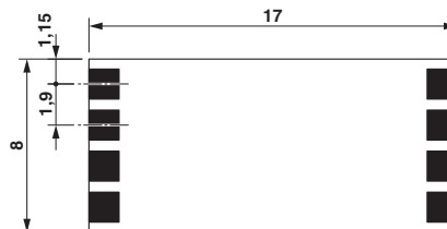
Dimensional drawing
