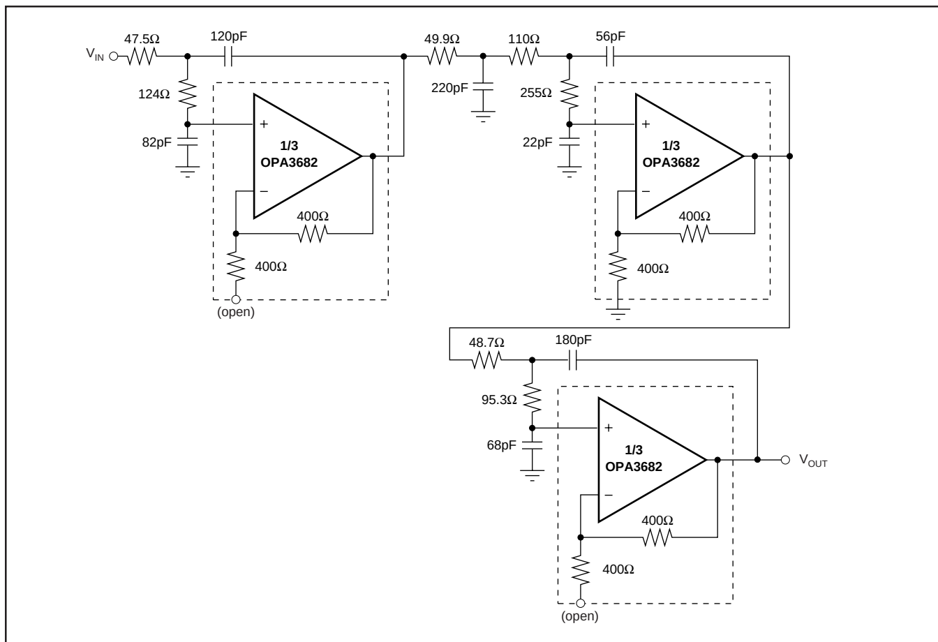
FIGURE 5. 7th-Order Butterworth Filter.
