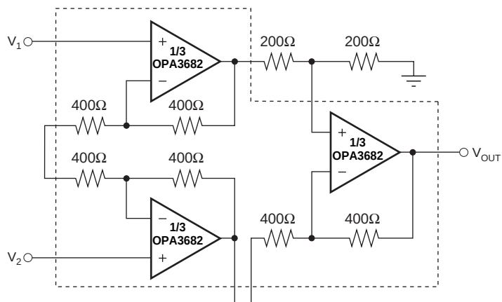
FIGURE 3. High-Speed Instrumentation Amplifier.
