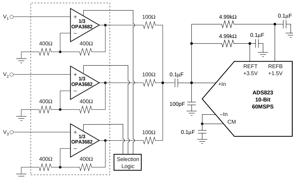
FIGURE 4. Multiplexed Converter Driver.
