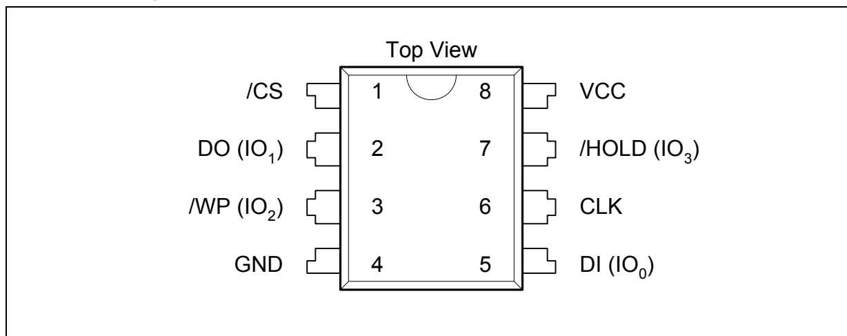
Figure 1c. W25Q16CV Pin Assignments, 8-pin PDIP (Package Code DA)
