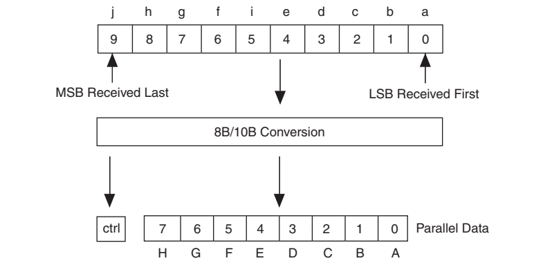
Figure 2–17. 10-Bit to 8-Bit Conversion
