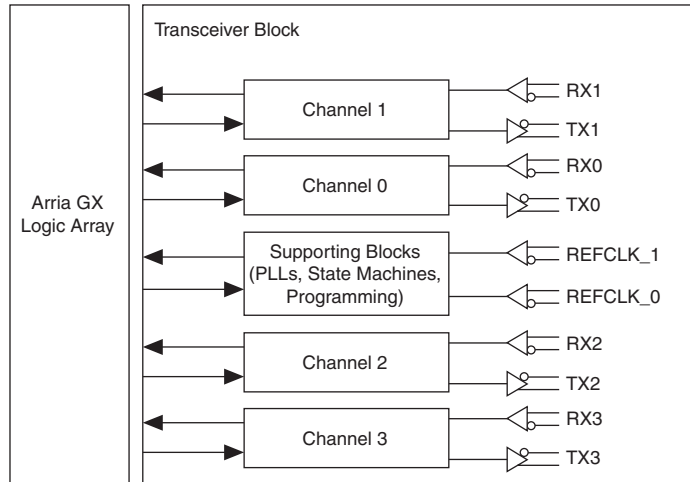
Figure 2–1. Transceiver Block
