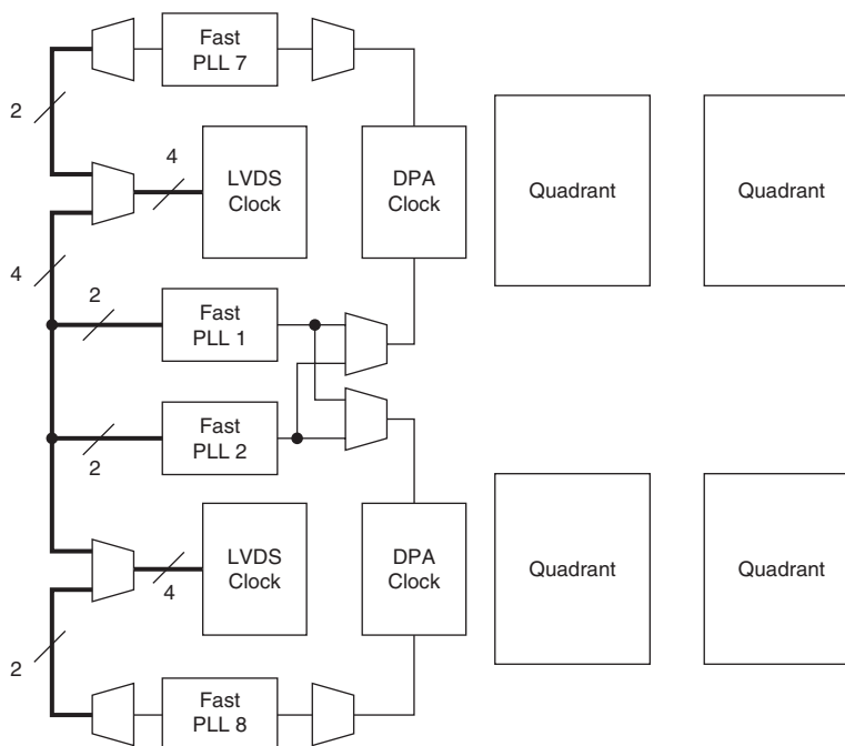
Figure 2–82. Fast PLL and Channel Layout in the EP1AGX60E and EP1AGX90E Devices Note (1)
