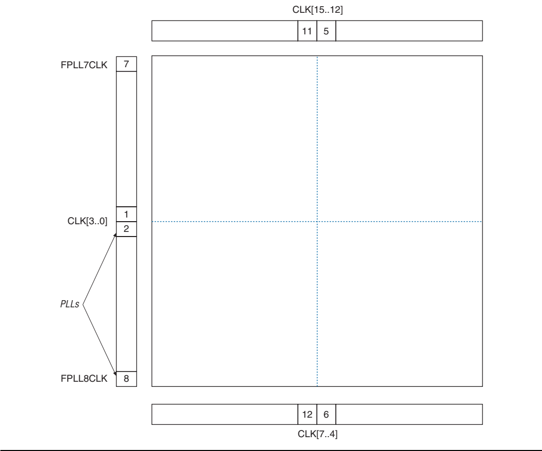
Figure 2–61. PLL Locations
