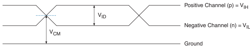
Figure 4–5. Receiver Input Waveforms for Differential I/O Standards
