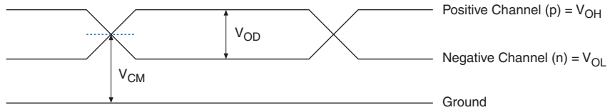
Figure 4–6. Transmitter Output Waveforms for Differential I/O Standards
