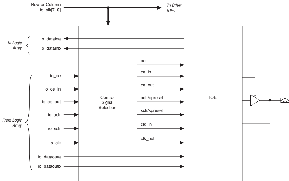
Figure 2–70. Signal Path Through the I/O Block
