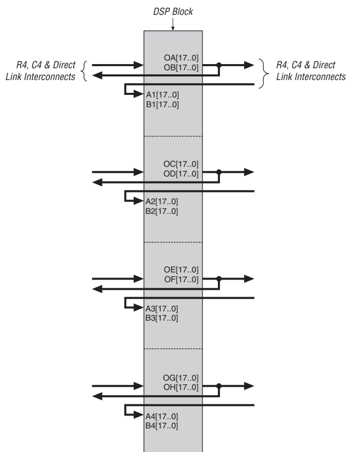
Figure 2–52. DSP Block Interconnect Interface
