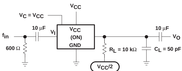
Figure 10. Sine-Wave Distortion
