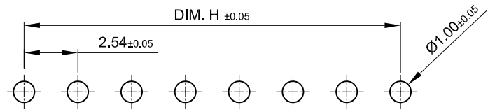
PCB Layout
