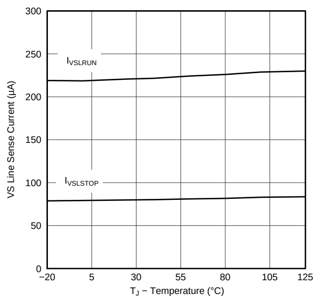
Figure 4. Line-Sense Current vs. Temperature
