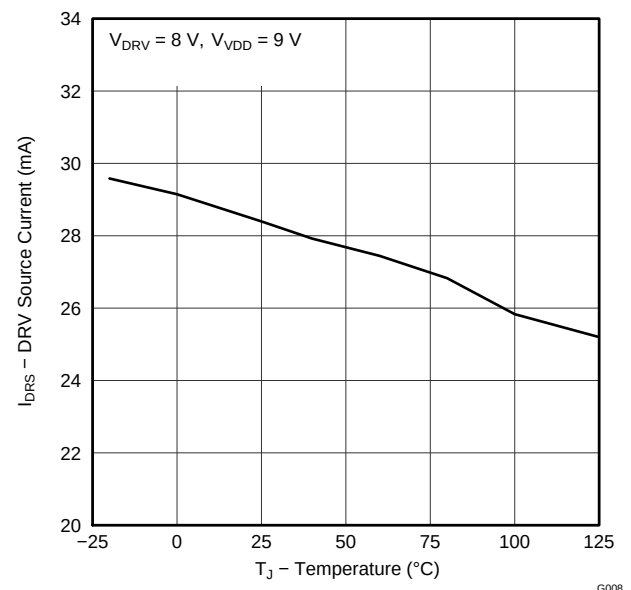
Figure 8. DRV Source Current vs. Temperature
