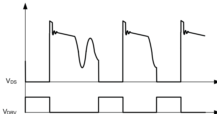
Figure 18. Valley-Skipping Mode
