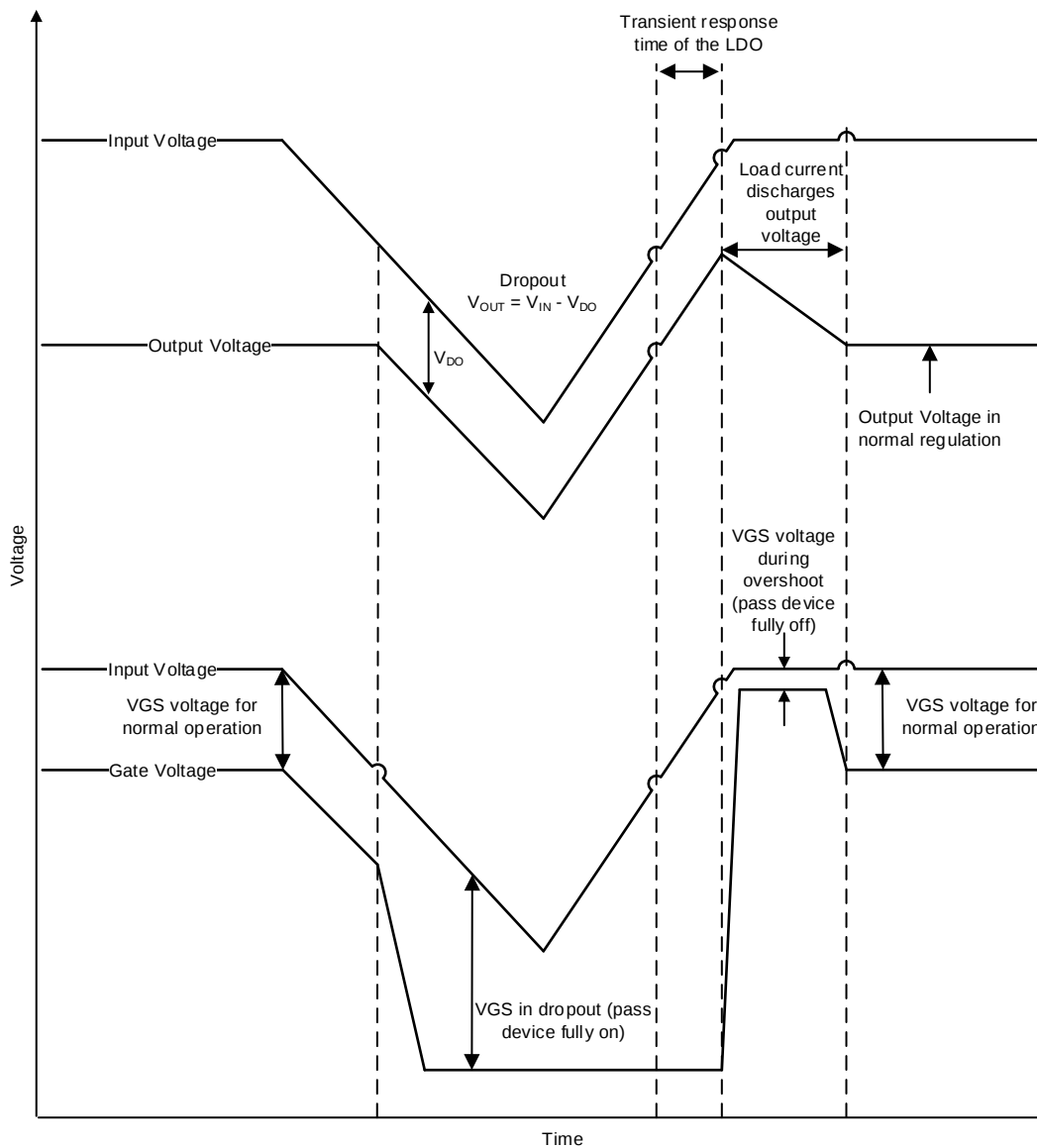
Figure 25. LDO Response Entering and Exiting Dropout
