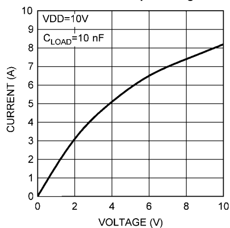
Sink Current vs. Output Voltage
