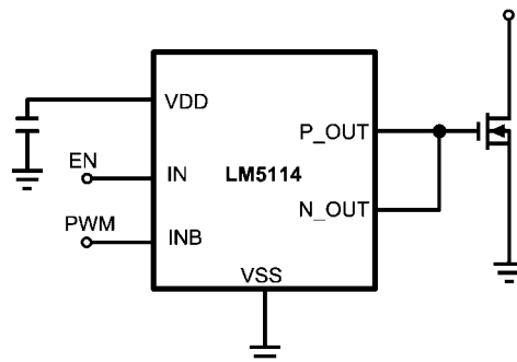
FIGURE 5. Inverting Application with Enable Pin
