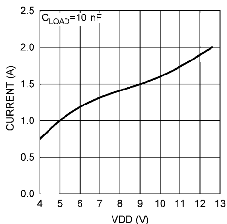
Peak Source Current vs. V DD Voltage
