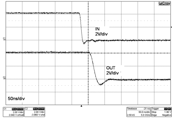
Input Voltage vs. Output Voltage ( V_{DD} = 4V , C_L = 10000pF )
