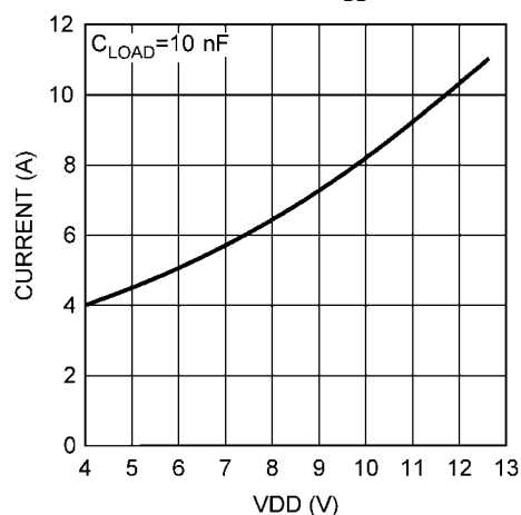
Peak Sink Current vs. V DD Voltage
