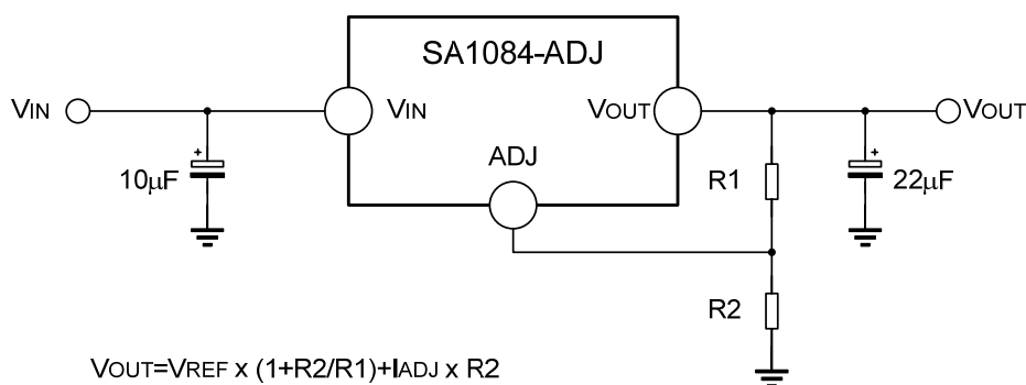
Figure 2. Typical Adjustable Output Voltage
